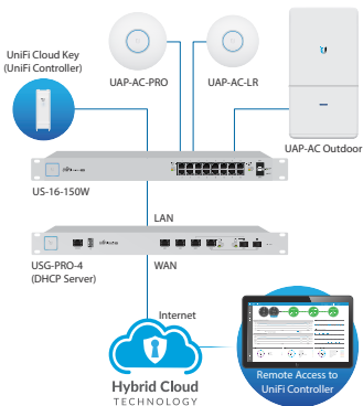
Sample Network Diagram
